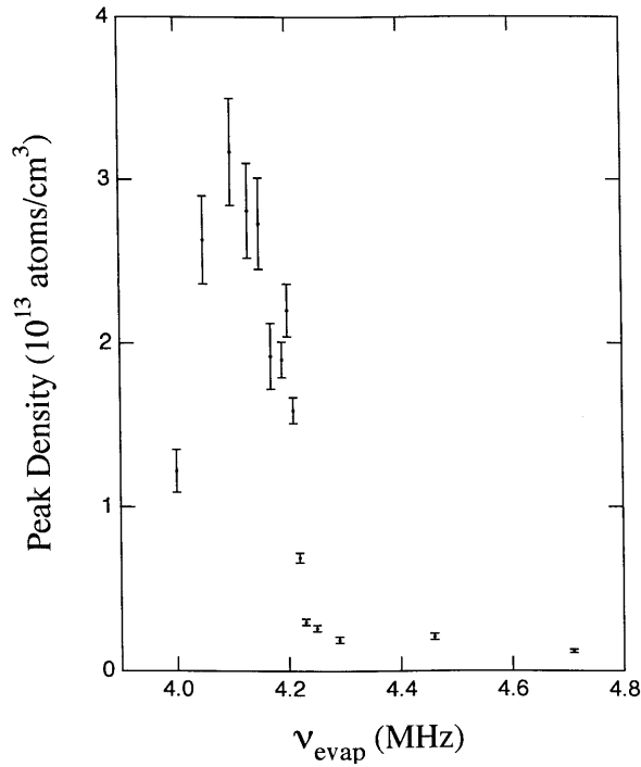
Fig. 5. Peak density at the center of the sample as a function of the final depth of the evaporative cut, \nu_{\text{evap}} . As evaporation progresses to smaller values of \nu_{\text{evap}} , the cloud shrinks and cools, causing a modest increase in peak density until \nu_{\text{evap}} reaches 4.23 MHz. The sudden discontinuity at 4.23 MHz indicates the first appearance of the high-density condensate as the cloud undergoes a phase transition. Source: M. H. Anderson, et al. (ref. 6), p. 200.
