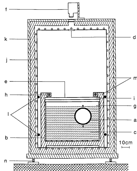
Fig. 7. Schematic diagram of the differential accelerometer used in Thieberger’s experiment. A precisely balanced hollow copper sphere (a) floats in a copper-lined tank (b) filled with distilled water (c). The sphere can be viewed through windows (d) and (e) by means of a television camera (f). The multiple-pane window (e) is provided with a transparent x - y coordinate grid for position determination on top with a fine copper mesh (g) on the bottom. The sphere is illuminated for one second per hour by four lamps (h) provided with infrared filters (i). Constant temperature is maintained by means of a thermostatically controlled copper shield (j) surrounded by a wooden box lined with Styrofoam insulation (m). The Mumetal shield (k) reduces possible effects due to magnetic field gradients and four circular coils (l) are used for positioning the sphere through forces due to ac-produced eddy currents, and for dc tests. Source: P. Thieberger, “Search for a Substance-Dependent Force with a New Differential Accelerometer” (ref. 10), p. 1067.
