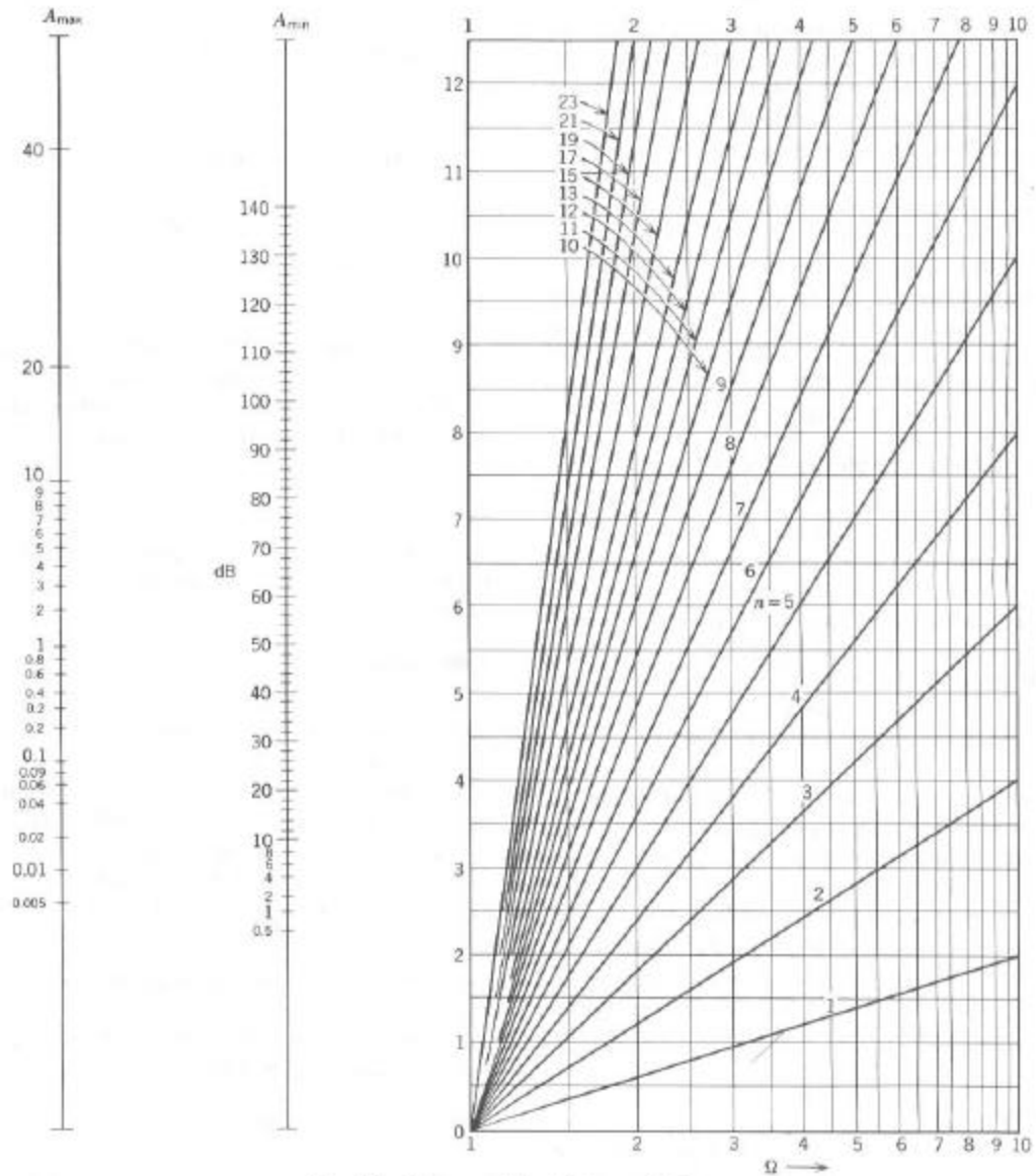
Fig. 5.1. Nomograph for Butterworth filters.
