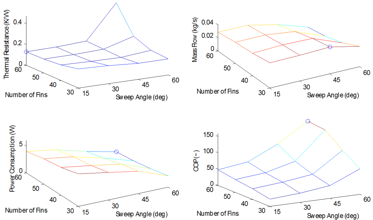
Figure 102: CFD parameter study results from batch 1 at 2500 rpm. The circle on each surface indicates the design with the optimal value.
