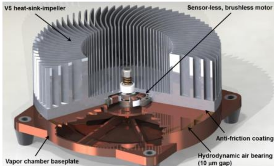
Figure 1. Sandia Cooler.
