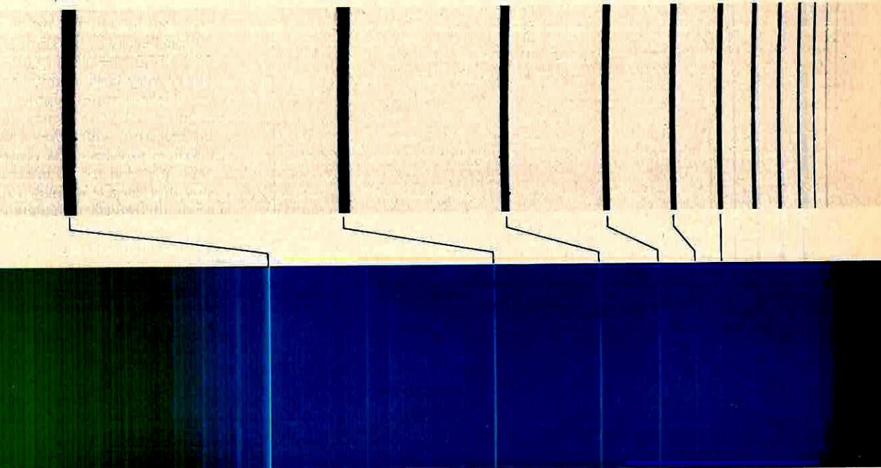
WAVELENGTH (ANGSTROM UNITS) BALMER-BETA BALMER-GAMMA BALMER-DELTA 4,861 4,340 4,102
